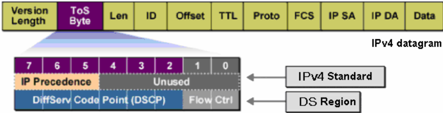
Figure 9-3 IP datagram
