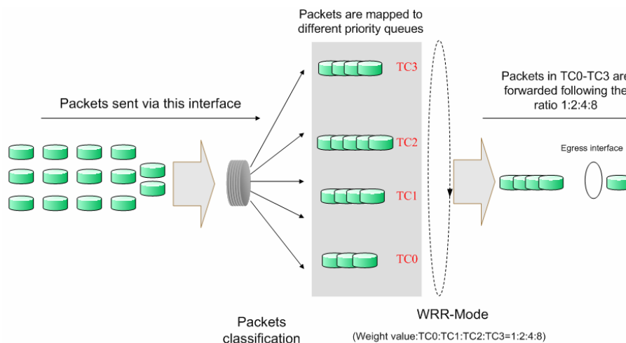
Figure 9-5 WRR-Mode
