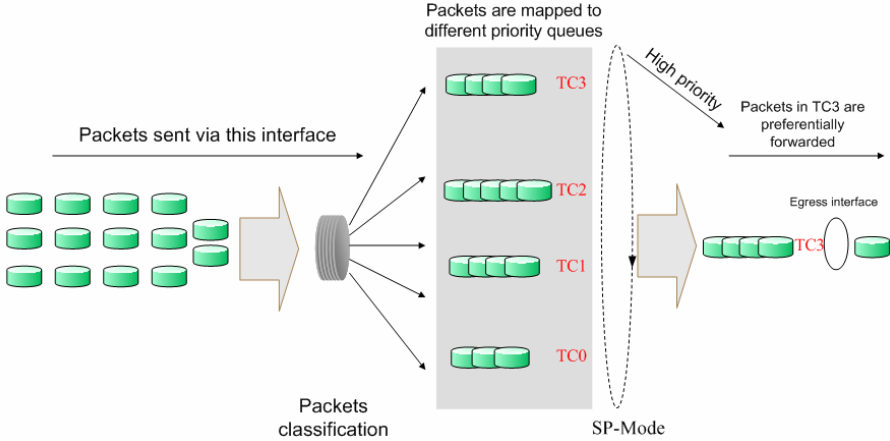
Figure 9-4 SP-Mode
