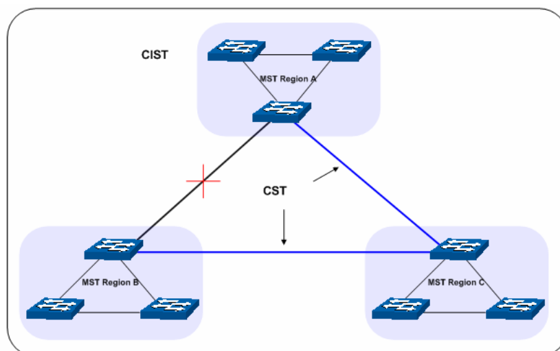
Figure 7-2 Basic MSTP diagram
