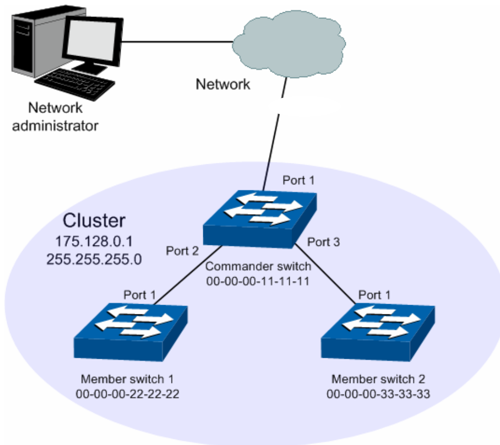
Figure 14-19 Network diagram
