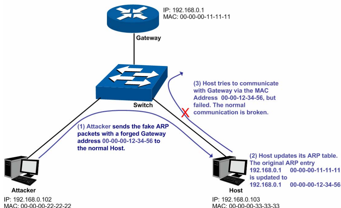
Figure 11-9 ARP Attack - Imitating Gateway
