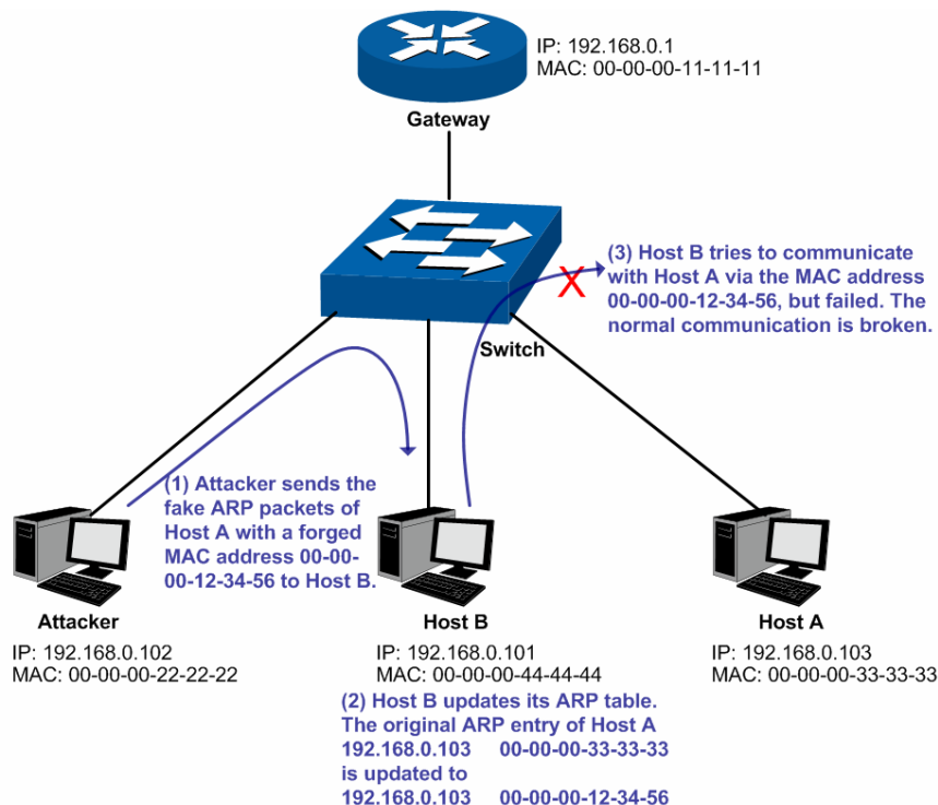
Figure 11-11 ARP Attack – Cheating Terminal Hosts
