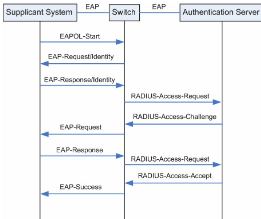
Figure 11-19 EAP-MD5 Authentication Procedure
