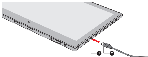
Figure 4-20 Connecting the HDMI Micro port
