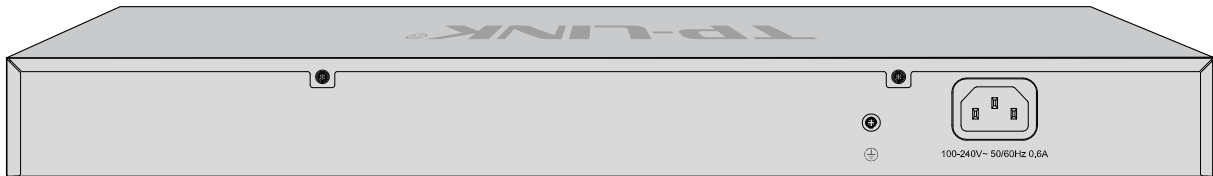
Figure 2-4 Rear Panel of TL-SL2428
